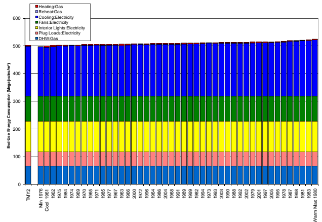
Figure 8 San Juan, Puerto Rico, Energy End-Use Consumption for 550 m 2 Office Building
